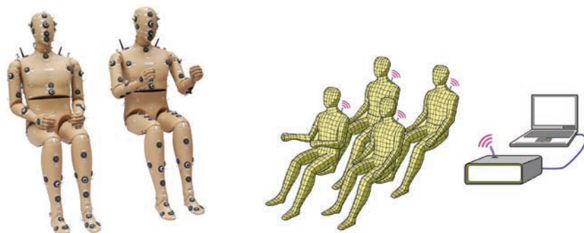
Measurement Software
