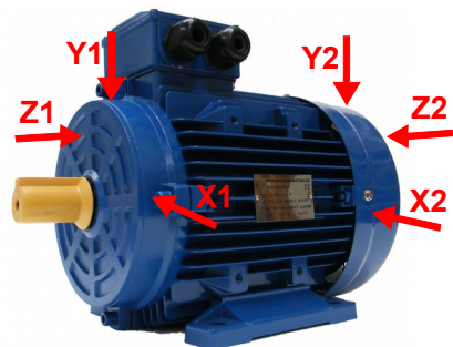
Figure 11: Measuring points on electric motors
