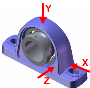
Figure 9: Measuring points on vertical bearings
